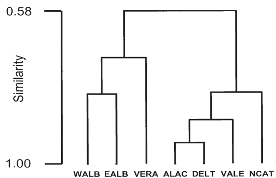
Fig. 2. – Dendrogram of similarities among geographical sectors based on their faunistic resemblance using Yule's similarity index and the UPGMA aggregation algorithm. WALB: Western Alborán Sea; EALB: Eastern Alborán Sea; VERA: Vera Gulf; ALAC: Alacant; EIVI: Eivissa Island; VALE: Valencia; DELT: Ebro delta region; NCAT: Northern Catalonia.
