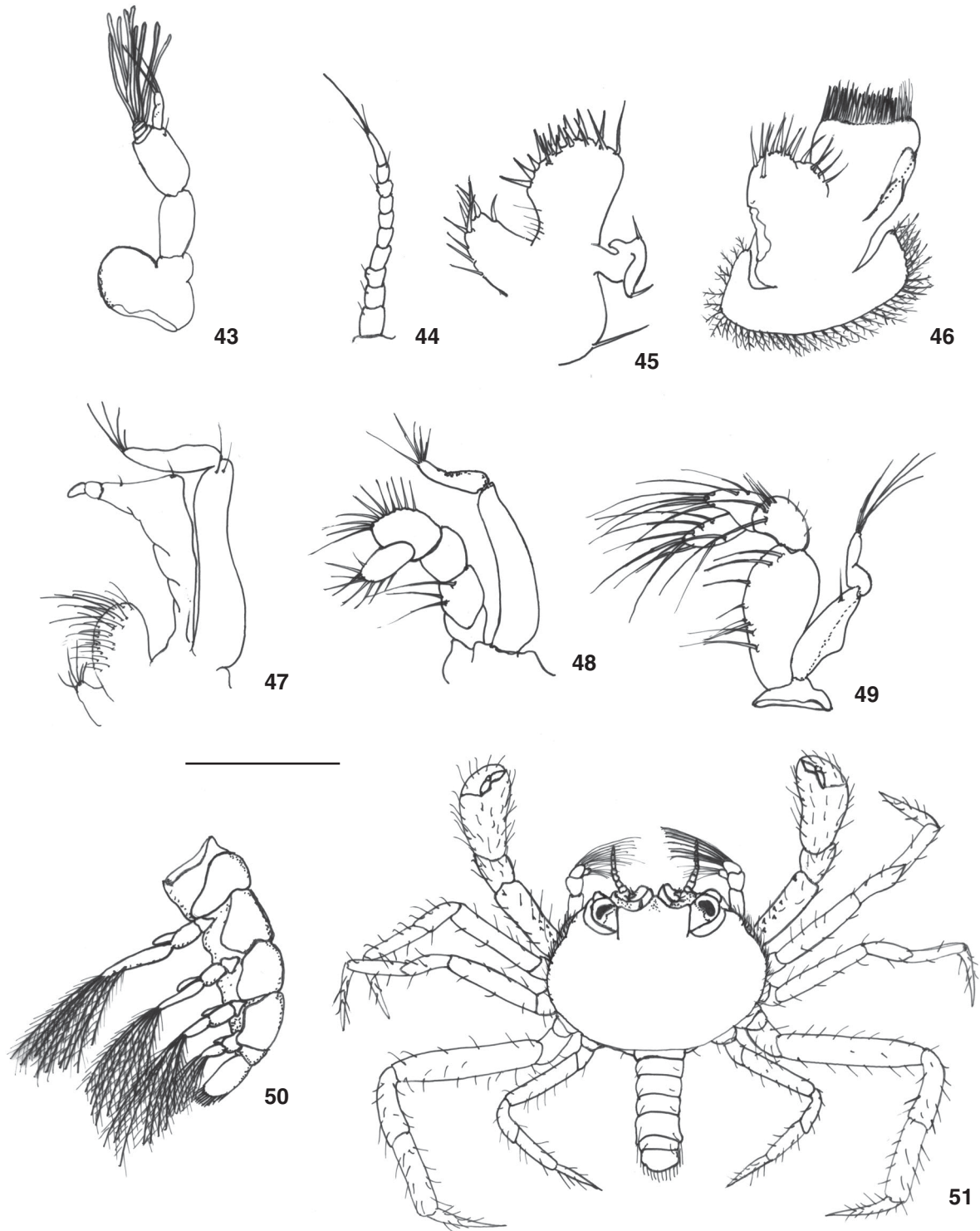
Figures 43-51. Megalopa of Pinnixa gracilipes : (43) antennule; (44) antenna; (45) maxillule; (46) maxilla; (47) first maxilliped; (48) second maxilliped; (49) third maxilliped; (50) abdomen and telson; (51) megalopa, dorsal view. Scale bar: 43-44 = 0.5 mm; 45-46 = 0.24 mm; 47-49 = 0.33 mm; 50 = 0.46 mm; 51 = 0.96 mm.
