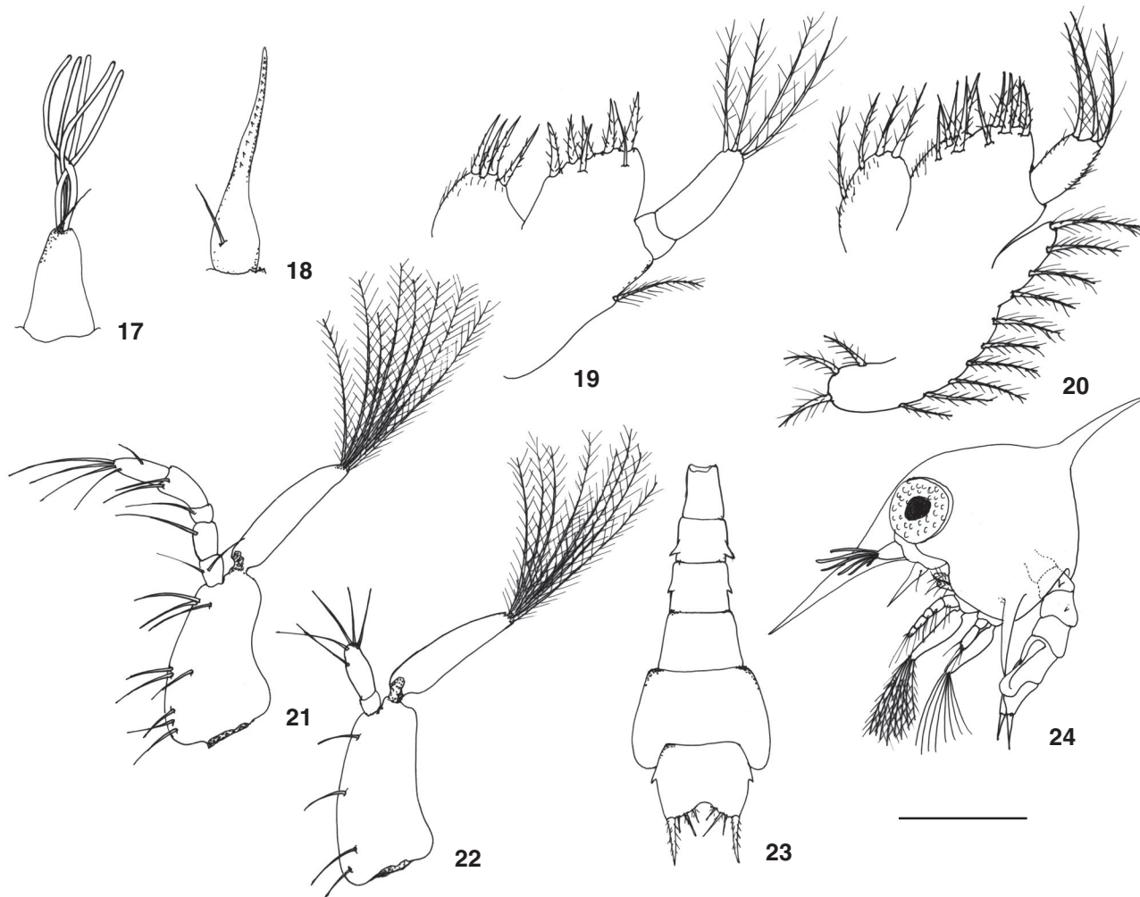
Figures 17-24. Zoea III of Pinnixa gracilipes : (17) antennule; (18) antenna; (19) maxillule; (20) maxilla; (21) first maxilliped; (22) second maxilliped; (23) abdomen and telson; (24) zoea III, lateral view. Scale bar: 17-20 = 0.85 mm; 21-22 = 0.15 mm; 23 = 0.25 mm; 24 = 0.46 mm.
