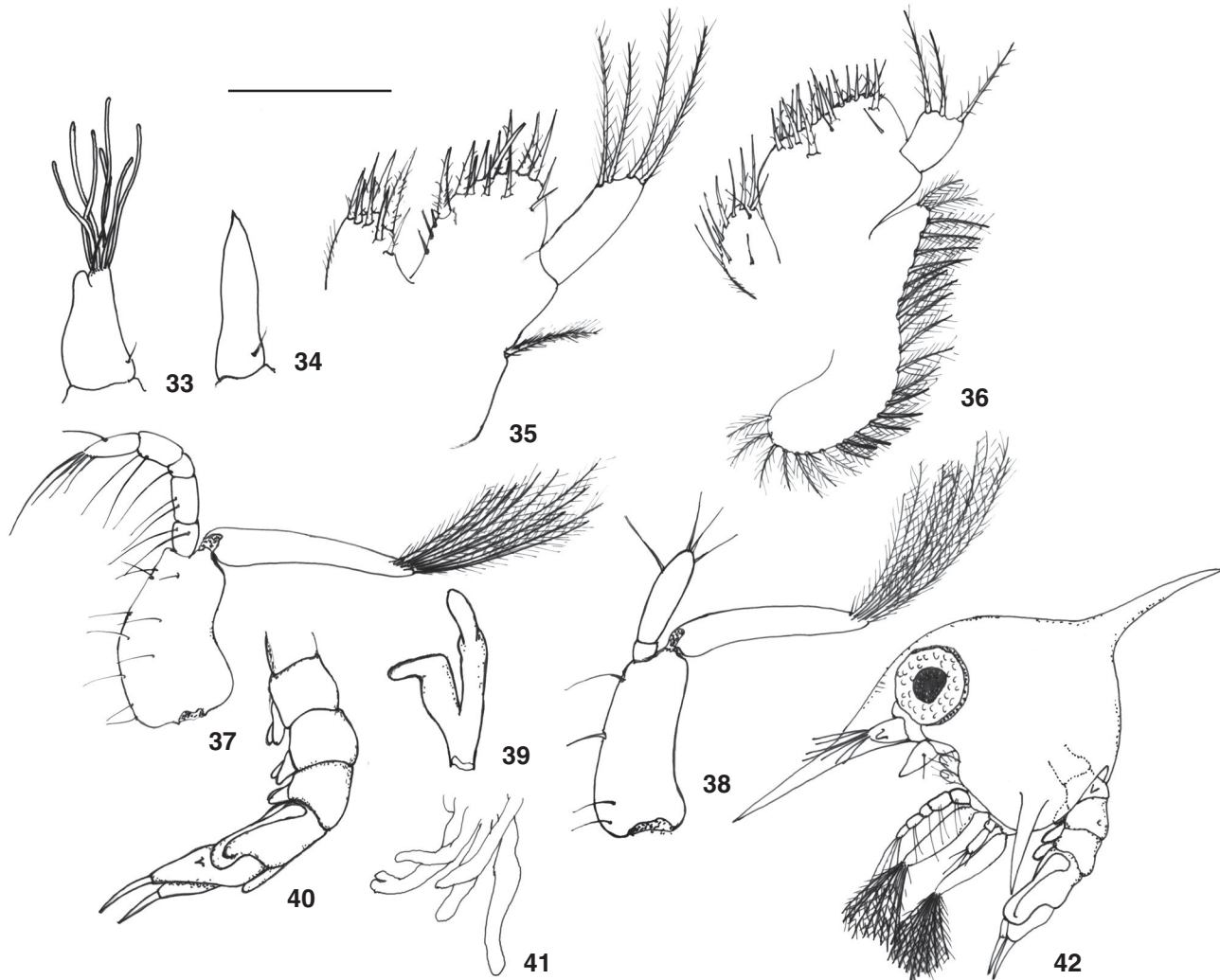
Figure 33-42. Zoea V of Pinnixa gracilipes : (33) antennule; (34) antenna; (35) maxillule; (36) maxilla; (37) first maxilliped; (38) second maxilliped; (39) third maxilliped; (40) abdomen and telson; (41) pereiopods; (42) zoea V, lateral view. Scale bar: 33-34 = 0.24 mm; 35-36 = 0.15 mm; 37-38 = 0.25 mm; 39 = 0.075 mm; 40 = 0,36 mm; 41 = 0,085 mm; 42 = 0.73 mm.
