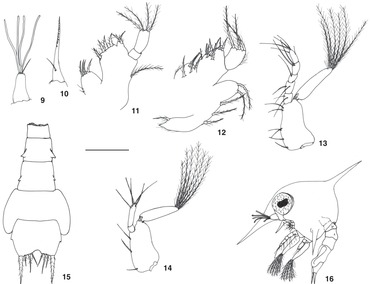
Figures 9-16. Zoea II of Pinnixa gracilipes . (9) antennule; (10) antenna; (11) maxillule; (12) maxilla; (13) first maxilliped; (14) second maxilliped; (15) abdomen and telson; (16) zoea II lateral view. Scale bar: 9-12 = 0.075 mm; 13-14 = 0.15 mm; 15 = 0.2 mm; 16 = 0.36 mm.
