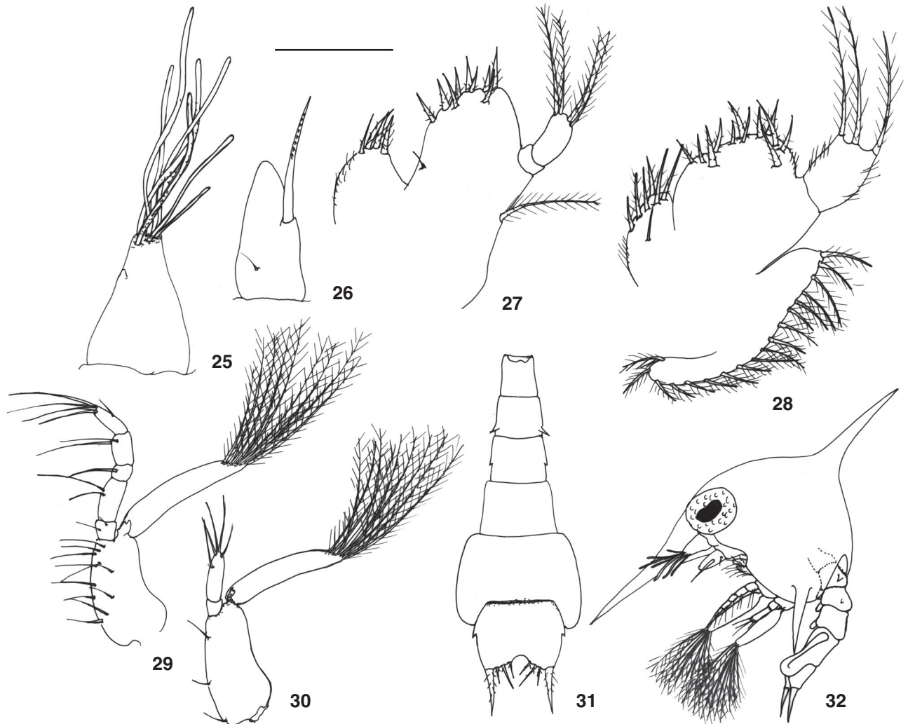
Figures 25-32. Zoea IV of Pinnixa gracilipes : (25) antennule; (26) antenna; (27) maxillule; (28) maxilla; (29) first maxilliped; (30) second maxilliped; (31) abdomen and telson; (32) zoea IV, lateral view. Scale bar: 25-28 = 0.1 mm; 29-30 = 0.2 mm; 31 = 0.3 mm; 32 = 0.6 mm.
