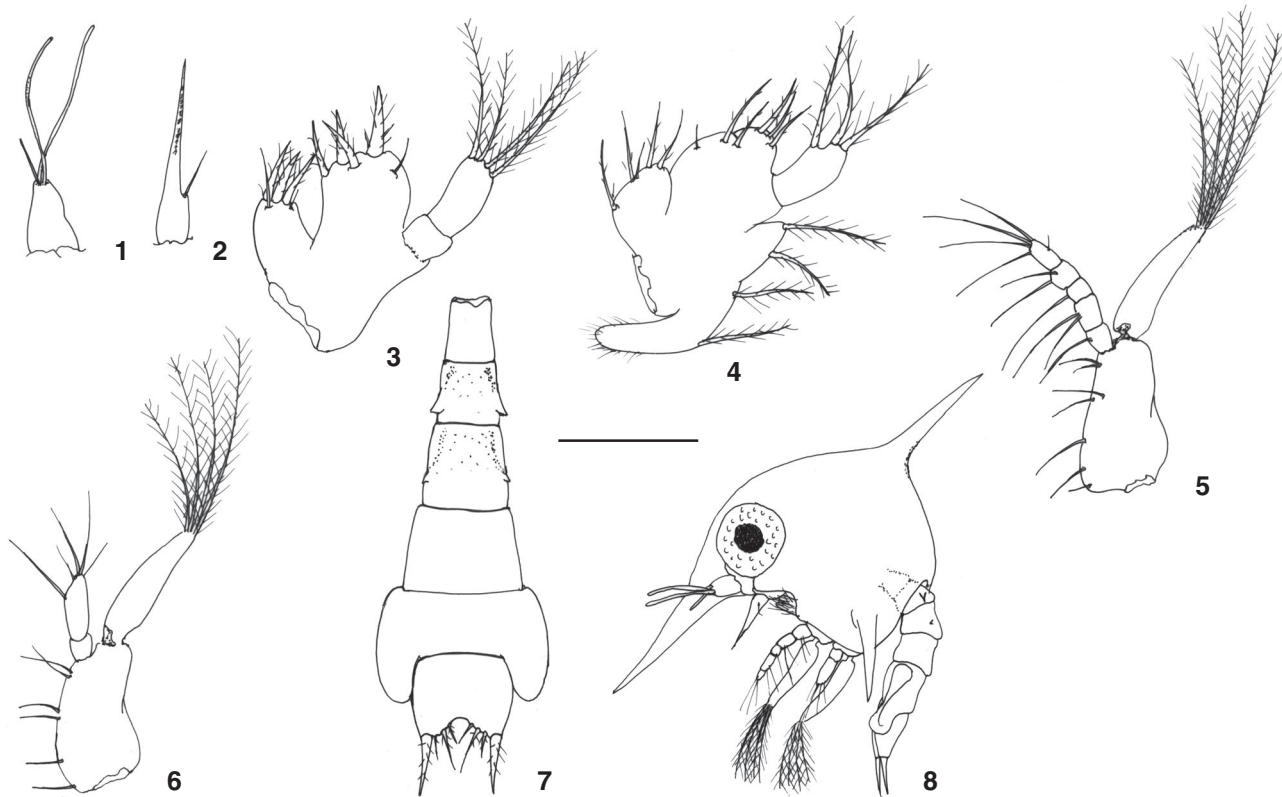
Figures 1-8. Zoea I of Pinnixa gracilipes : (1) antennule; (2) antenna; (3) maxillule; (4) maxilla; (5) first maxilliped; (6) second maxilliped; (7) abdomen and telson; (8) first zoea lateral view. Scale bar: 1-4 = 0.075 mm; 5-6 = 0.15 mm; 7 = 0.2 mm; 8 = 0.3 mm.
