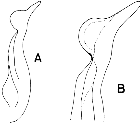
Fig. 53. Thaipotamon spec., ♂, left G1 (43.0 by 32.0 mm) (USNM 94414) (copied from photographs). A, ventral view; B, terminal segment.
