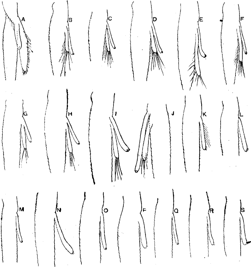
Fig. 28. Endopodite of second abdominal appendage of male (A~J) and female (K~S). A and P, L. paucidens , \times 12 ; B and K, L. serrifer , \times 20 ; C and L, L. macrodactylus , \times 16 ; D ( \times 12 ) and M ( \times ca. 8), L. gravieri ; E and N, L. longicarpus , \times 28 ; F ( \times 12 ) and O ( \times 16 ), L. longipes ; G and Q, L. modestus ; H and S, L. japonicus ; I ( \times 12 ) and R ( \times ca. 8), L. carinatus ; J, L. stylirostris , \times 16 ; P, L. gravieri , \times 16 .
