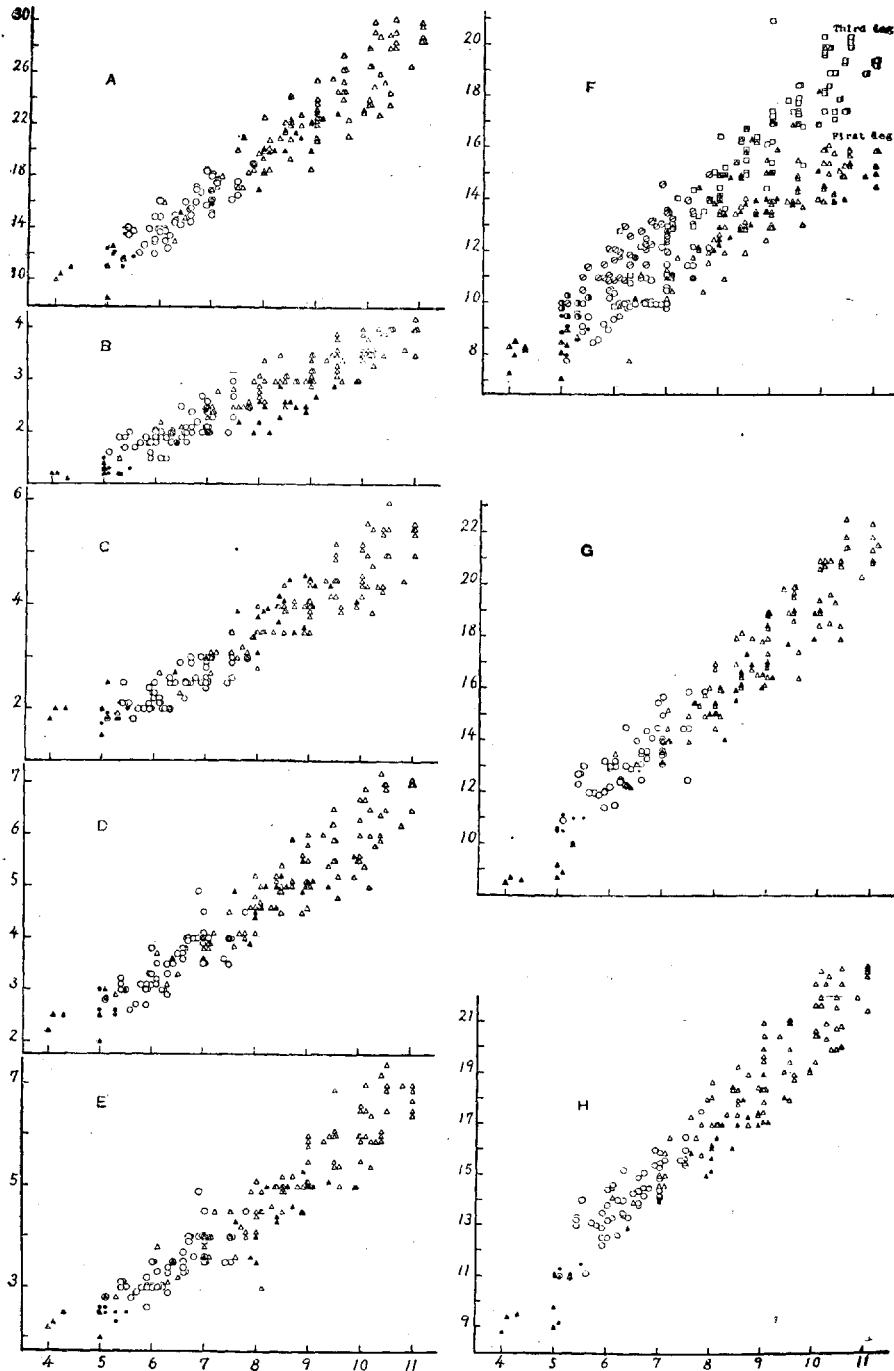
Fig. 8. Length (in mm) of second leg (A) and finger (B), palm (C), carpus (D) and merus (E) of second pereiopod, first, third (F), fourth (G) and fifth (H) pereiopods in relation to carapace-length (in mm). ● and ○, ♂ and ♀ of L. serrifer ; ○ and ⊙, ♂ and ♀ of L. macrodactylus .
