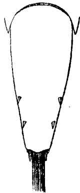
Fig. 1. Telson, \times 25 .
