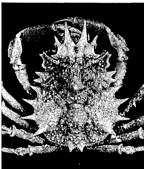
Fig.7a-c. Leptomithrax depressus n.sp., male holotype, 19.6 x 19.6 mm, AM P39425. a: general view; b: dorsal view; c: pleopod 1 (length, 3.2 mm).
