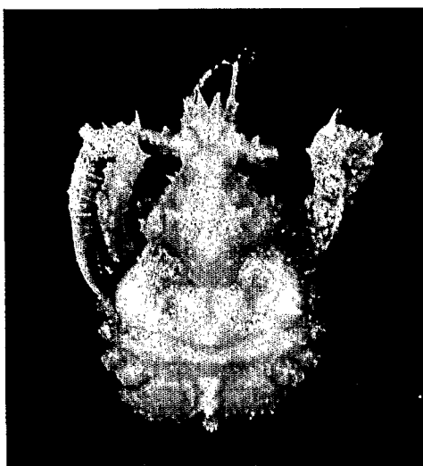
Fig.3a,b. Achaeus curvirostris . a: female, ovigerous, 5.4 x 4.5 mm AM P39424; b: male, 4 x 3 mm, AM P40737.
