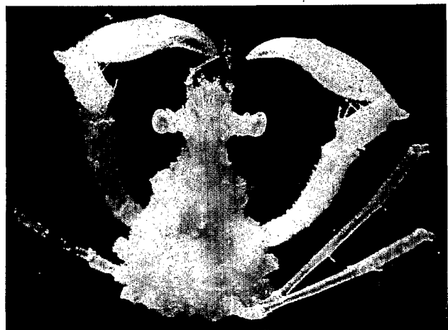
Fig.3a,b. Achaeus curvirostris . a: female, ovigerous, 5.4 x 4.5 mm AM P39424; b: male, 4 x 3 mm, AM P40737.
