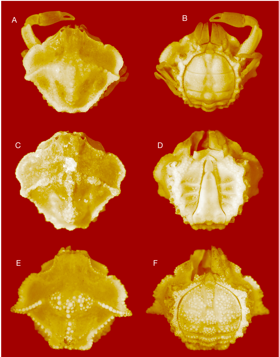
FIG. 4. — A-D , Nobiliella jousseaumei (Nobili, 1905) n. comb.; A, B , lectotype, ovig. ♀ 6.7 × 7.5 mm (MNHN B 17008) from Red Sea and Perim in dorsal and ventral views; C, D , allotype, ♂ 5.9 × 6.6 mm (MNHN B 28616) from Red Sea and Perim in dorsal and ventral views; E, F , Nobiliella cornigera (Nobili, 1905) n. comb., lectotype, ♀ 4.3 × 5.2 mm (MNHN B 17010) from Red Sea in dorsal and ventral views.
