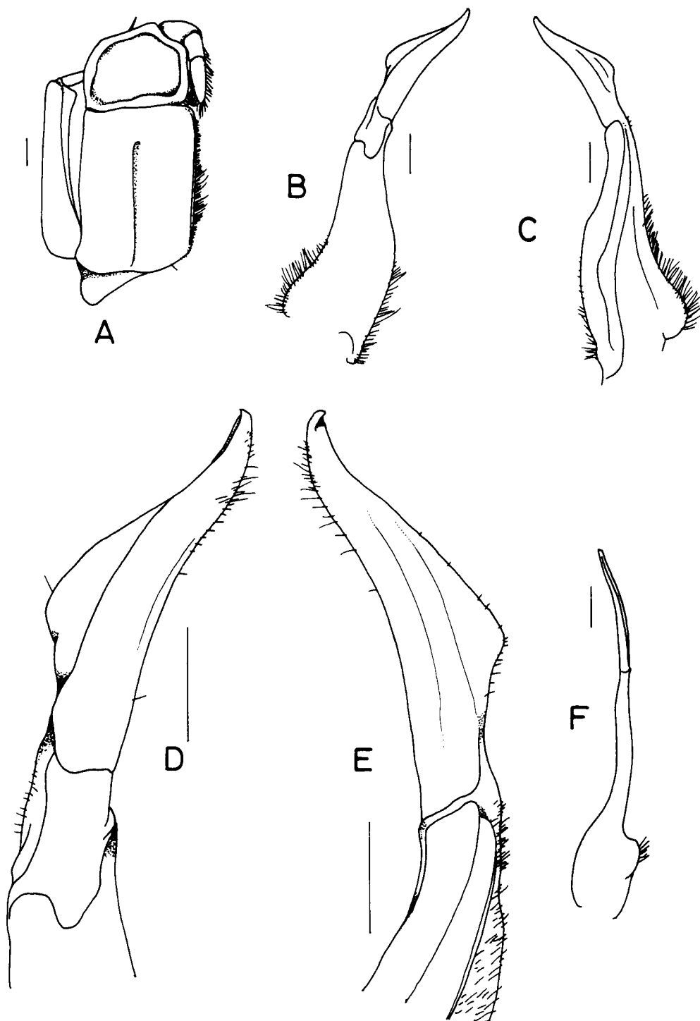
Fig. 58. Demanietta tritrunensis (Naiyanetr, 1986), paratype, ♂ (37.7 by 28.0 mm) (ZRC 1991.1857). A, right third maxilliped; B-E, right G1; F, right G2. B, D, dorsal view; C, E, ventral view; D, E, G1 terminal segment. Scales: 1.0 mm.
