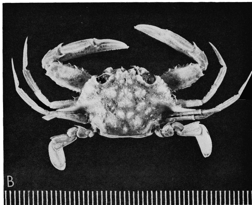
Portunus rugosus (A. Milne Edwards): A, form I, juv., Philippines, Sta. 5158, Albatross ; B, form II, male, Philippines, Sta. 5159, Albatross . (Scale 1 mm.)
